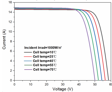
I-V characteristics at different temperatures (KS-N16/156HG650W)
